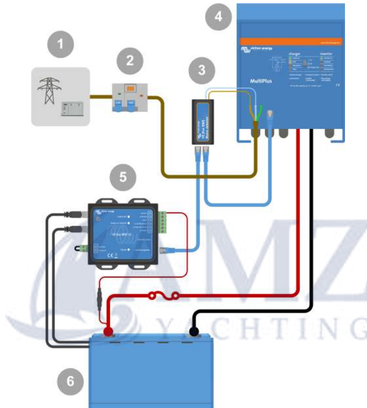
AC detector wiring example.
